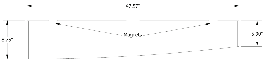
PROGRESSIVE WAVE 9" TO 6" DESIGN IN 9MM FOR 48" ACT GRID
