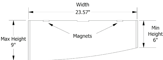
PROGRESSIVE WAVE 9" TO 6" DESIGN IN 18MM FOR 24" ACT GRID
