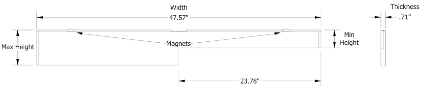
STEP DESIGN IN 18MM FOR 48" ACT GRID
