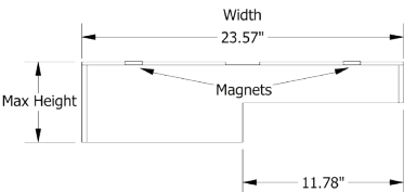
STEP DESIGN IN 18MM FOR 24" ACT GRID
