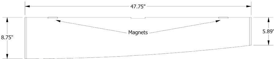
PROGRESSIVE WAVE 9" TO 6" DESIGN IN 18MM FOR 48" ACT GRID
