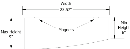
PROGRESSIVE WAVE 9" TO 6" DESIGN IN 9MM FOR 24" ACT GRID
