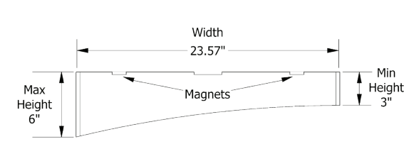
PROGRESSIVE WAVE 6" TO 3" DESIGN IN 18MM FOR 24" ACT GRID
