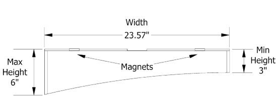
PROGRESSIVE WAVE 6" TO 3" DESIGN IN 9MM FOR 24" ACT GRID
