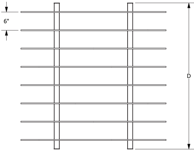
UNDERSIDE VIEW
