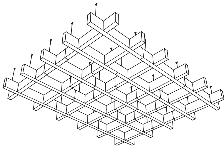
10'x12' - OPEN FRAME 24" SQUARE CELL
