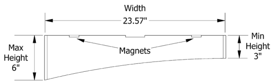
PROGRESSIVE WAVE 6" TO 3" DESIGN IN 18MM FOR 24" ACT GRID
