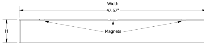
RECTANGLE DESIGN IN 9MM FOR 48" ACT GRID
