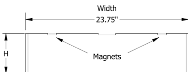
RECTANGLE DESIGN IN 18MM FOR 24" ACT GRID
