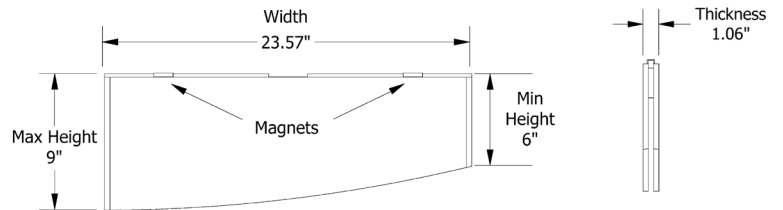
PROGRESSIVE WAVE 9" TO 6" DESIGN IN 9MM FOR 24" ACT GRID
