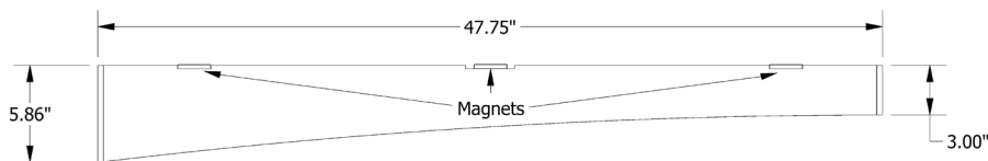
PROGRESSIVE WAVE 6" TO 3" DESIGN IN 18MM FOR 48" ACT GRID
