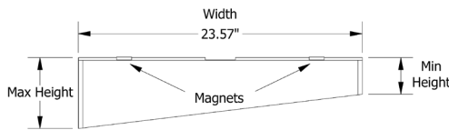
ANGLE DESIGN IN 9MM FOR 24" ACT GRID
