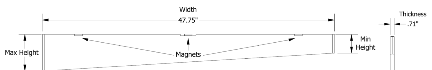
ANGLE DESIGN IN 18MM FOR 48" ACT GRID
