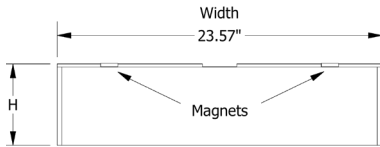
RECTANGLE DESIGN IN 9MM FOR 24" ACT GRID
