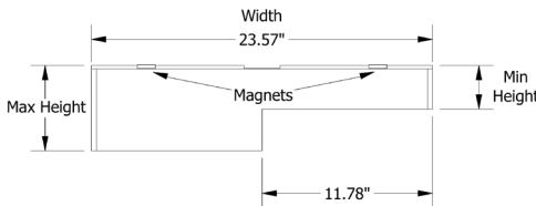
STEP DESIGN IN 9MM FOR 24" ACT GRID
