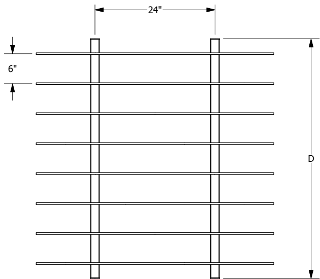
UNDERSIDE VIEW
