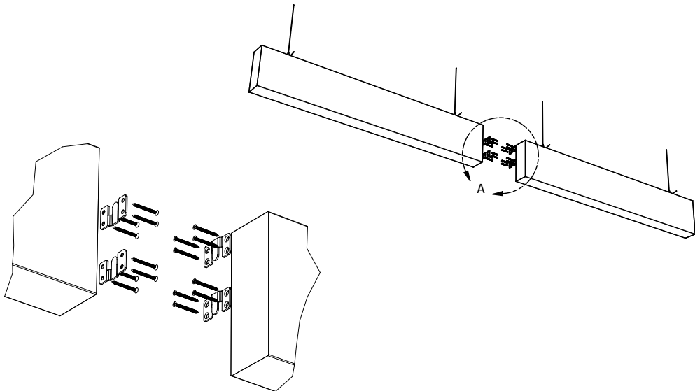
BEAM BAFFLE CONNECTORS (FOR SINGLE BEAMS ONLY) EBB-CONN
