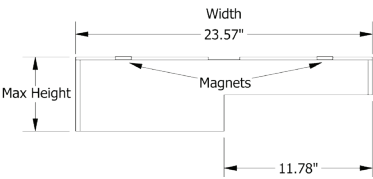
STEP DESIGN IN 18MM FOR 24" ACT GRID
