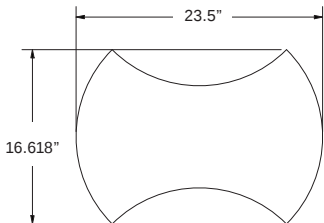
BOW-TIE - 24" (Dimensions Actual)
