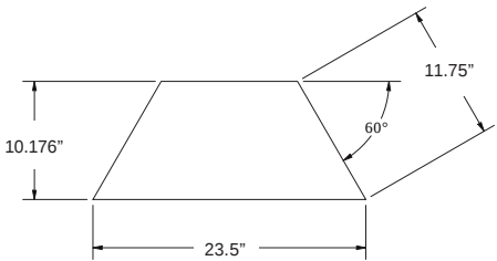
TRAPEZOID - 24" (Dimensions Actual)
