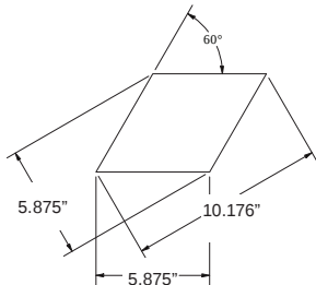
DIAMOND - 10" (Dimensions Actual)
