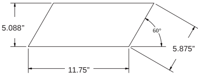
PARALLELOGRAM - 12" (Dimensions Actual)
