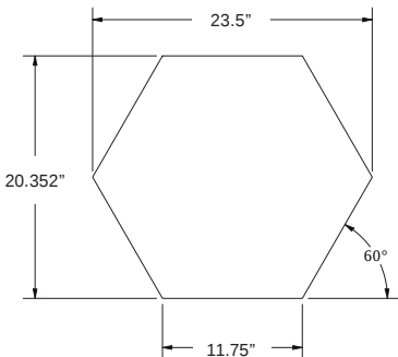
HEXAGON - 24" (Dimensions Actual)
