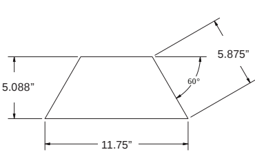
TRAPEZOID - 12" (Dimensions Actual)
