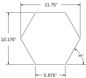
HEXAGON - 12" (Dimensions Actual)
