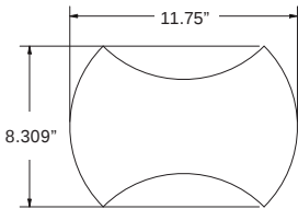
BOW-TIE - 12" (Dimensions Actual)
