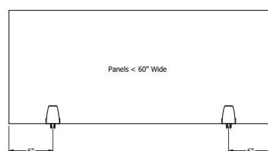
Stackers™ Flush Mount Panel (STKNS-PE9) with 90° square corners
