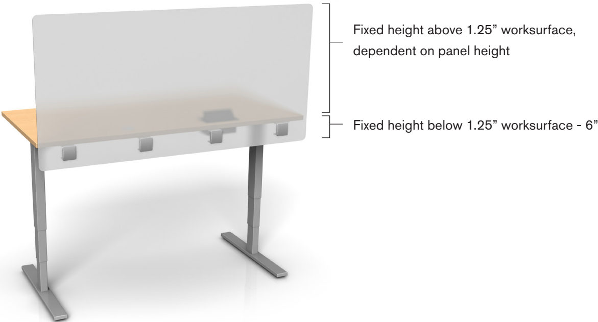
OPTION 2 6" Below the worksurface
